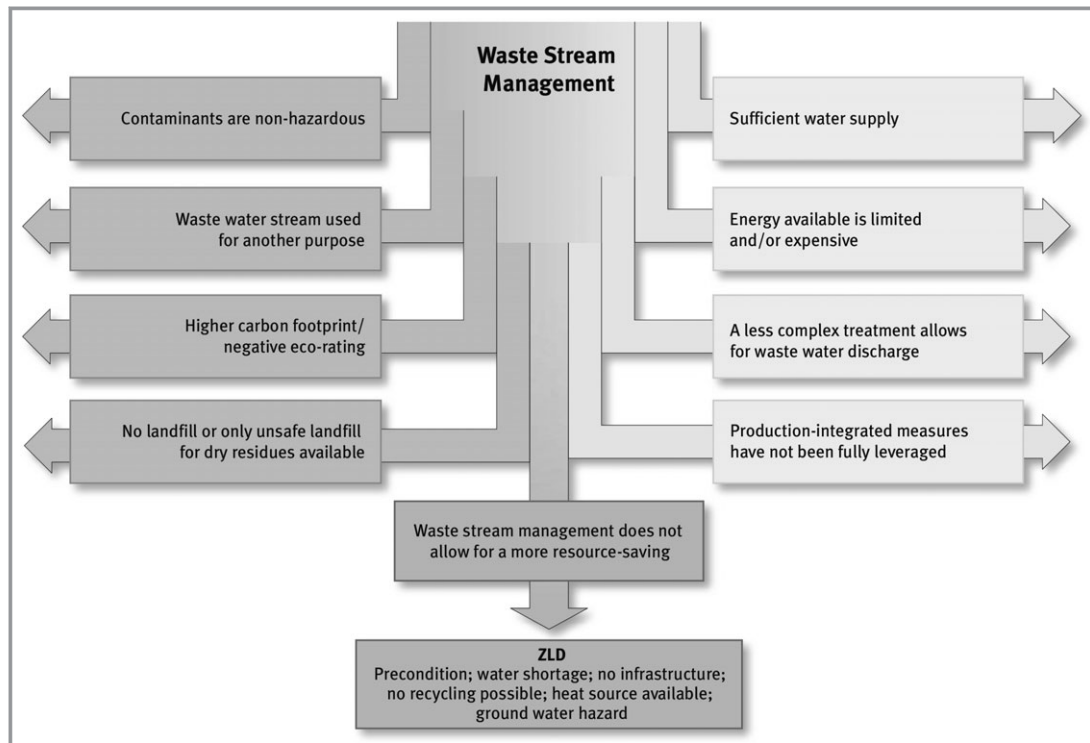
Figure 3. Drivers and benefits of zero liquid discharge (ZLD), reprint from [29].
