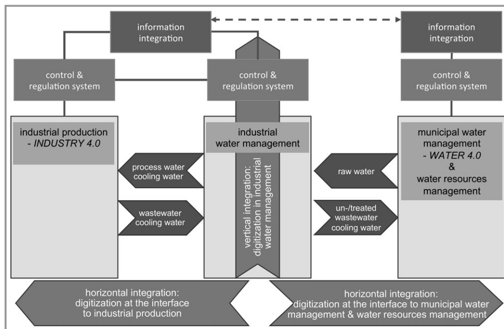
Figure 4. The integration of Industrial Water 4.0 (Industriewasser 4.0) in industrial production and municipal/water resources management, modified from [34].
